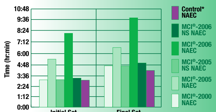
Average Setting Time, MCI® vs. Control*, Non-Air Entrained Concrete MCI Set Time Vs. Control (Non-Air Entrained Concrete)
