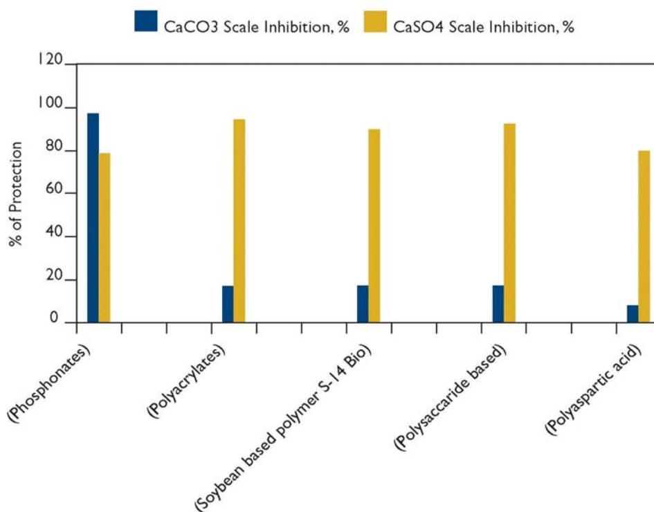
FIGURE 2 - Scale Inhibition (% of Protection)
