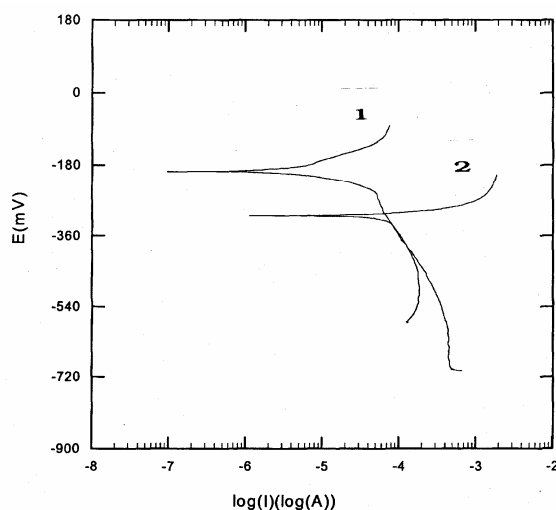
FIGURE 1 - Tafel plots. 1 - 300ppm S-10 F in de-ionized water; 2 – De-ionized water. Ambient temperature, 200 rpm.
