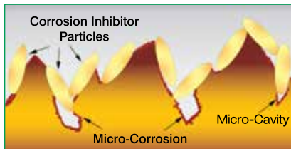
Traditional coatings can not protect the micro-cavities due to the relative large size of corrosion inhibitor particles such as nitrate, aluminum, zinc, and so on. That's where micro-corrosion starts when using traditional coatings.
