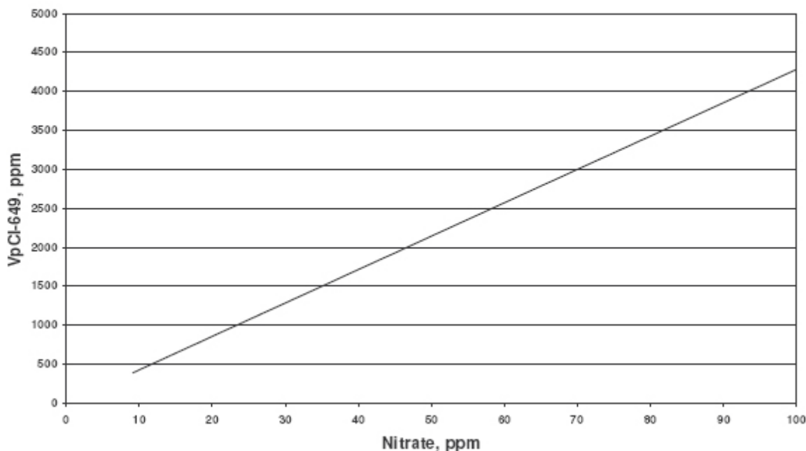
Theoretical Concentration of VpCI-649 vs Nitrate
