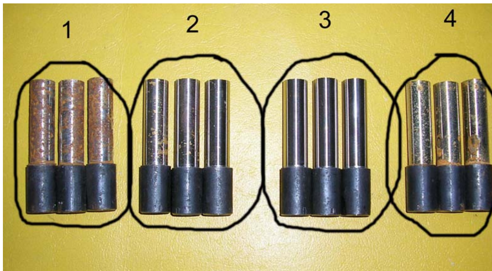
Figure 2. Appearance of samples machined without application of coolant (dry machining) after testing: 1-in salt chamber, 2-in atmospheric conditions, 3-in closed area, 4-in wet chamber.
