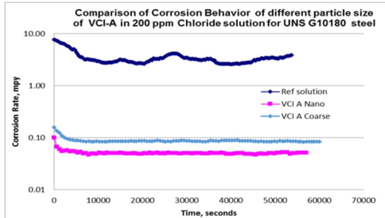
Comparison of corrosion behavior of different particle size for VCI-A in 200 ppm chloride solution for UNS G10180 steel.
