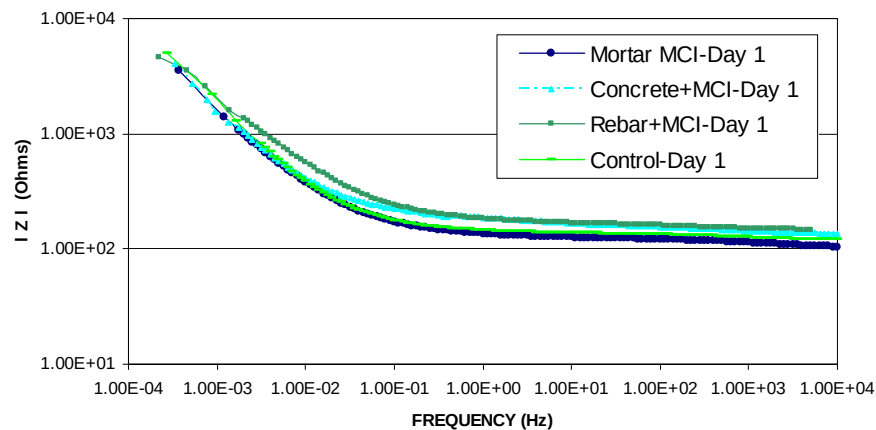
Figure 6. EIS Node plot for MCI 2022 treated & untreated concrete on day 1 of testing.
