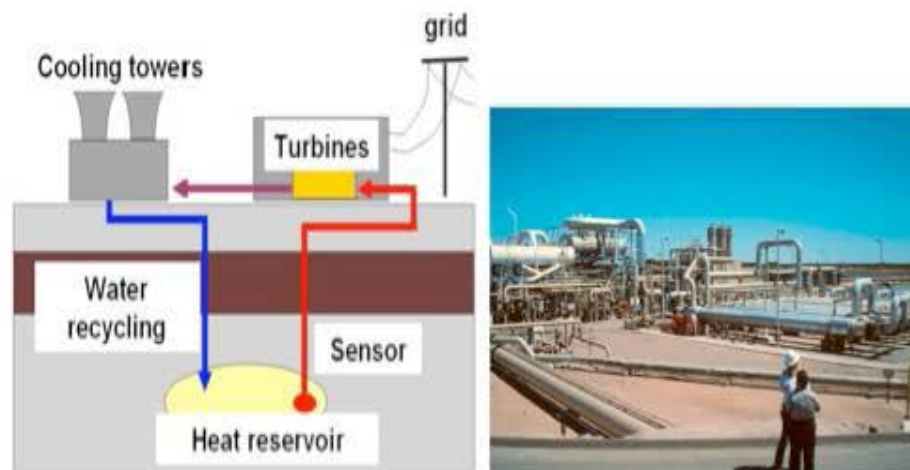
Figure 16: Geothermal power plant.
