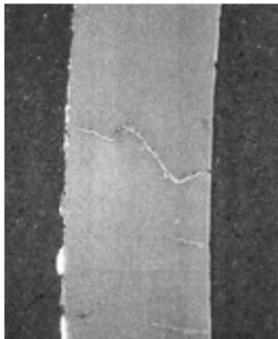
Figure 15: Stress corrosion cracking of carbon steel in biofuel. 25
